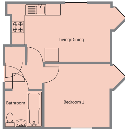
One Bedroom Apartment 35m 2 Apartment 1: Upper Ground Floor.
